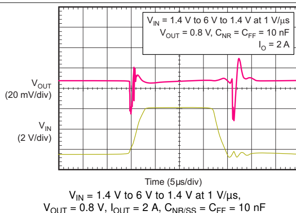
Figure 49. Line Transient
