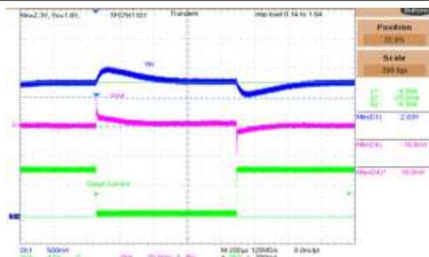
Figure 8-8. Load Transient Response: Step Load 0.1 to 1.6 A, V_{IN} = 2.3 V, V_{OUT} = 1.8 V
