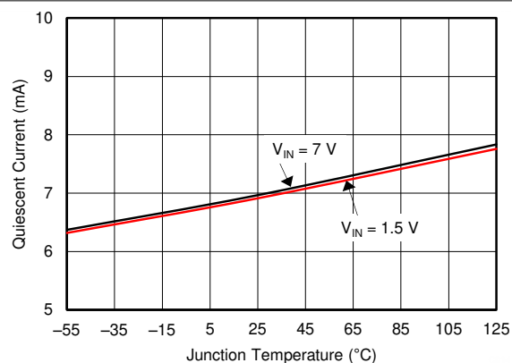
Figure 6-2. Quiescent Current vs Temperature
