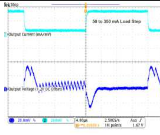
Figure 32. Load Transient Response in PFM/PWM Operation
