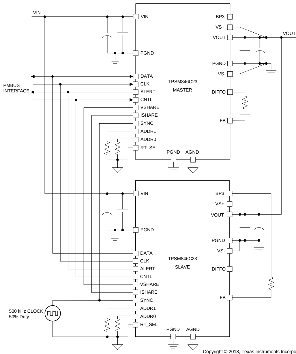
Figure 18. TPSM846C23 Parallel
