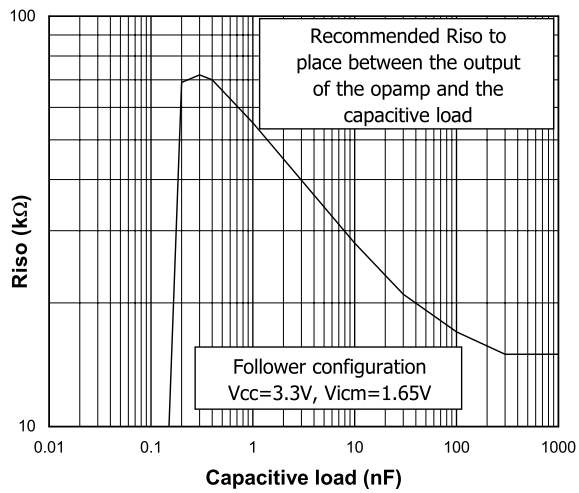
Figure 37. In series resistor R_{iso} vs. capacitive load
