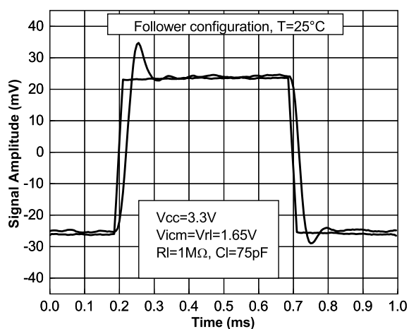
Figure 29. Small signal response at 3.3 V supply voltage
