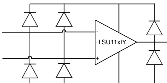
Figure 42. ESD structure
