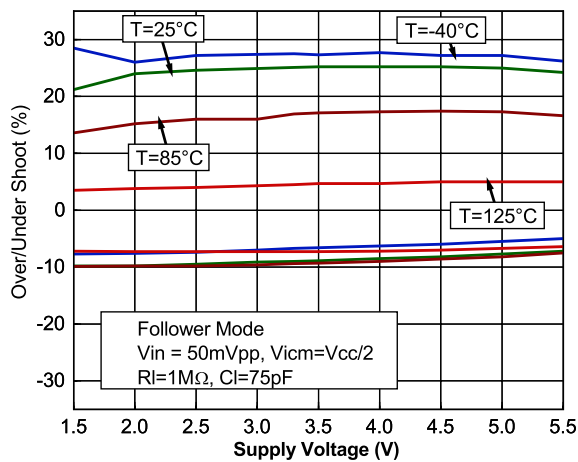
Figure 31. Over/under shoot vs supply voltage
