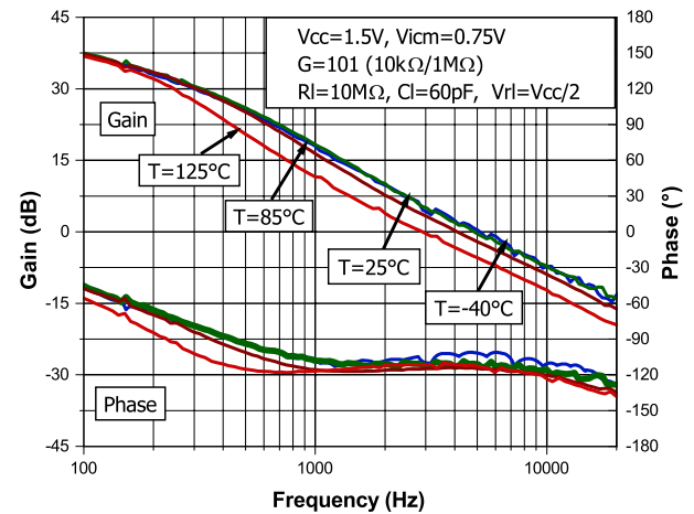
Figure 32. Bode diagram at 1.5 V supply voltage
