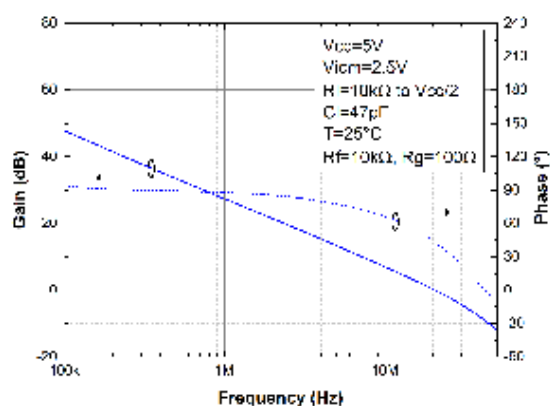
Figure 25. Closed loop bode diagram at V_{CC} = 5\text{ V}
