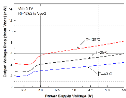
Figure 19. Output saturation voltage ( V_{OH} ) vs. supply voltage
