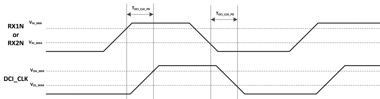
Figure 13. DCI Clock Propagation Delay
