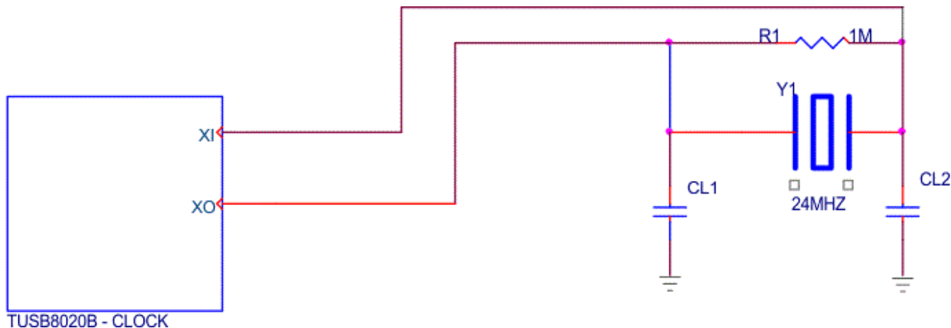
Figure 2. TUSB8020B Clock
