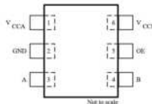
Figure 4-2. DBV, DCK, and DRL Package
