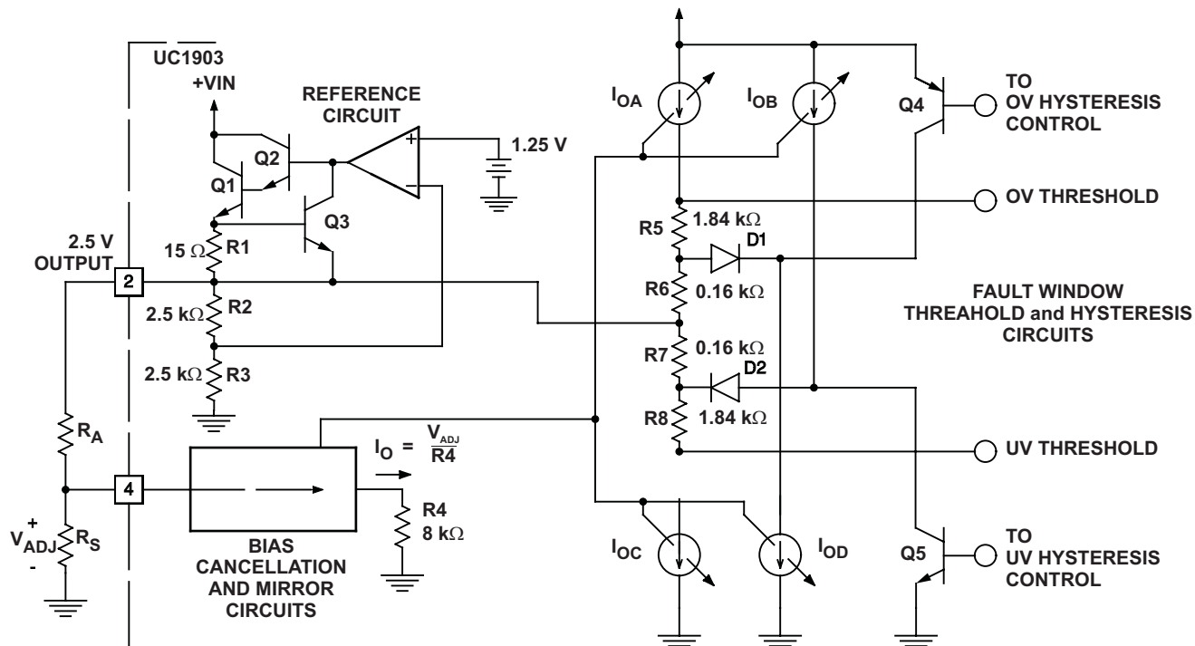
Block Diagram
