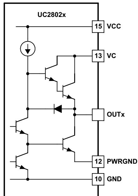
Figure 16. Simplified Schematic
