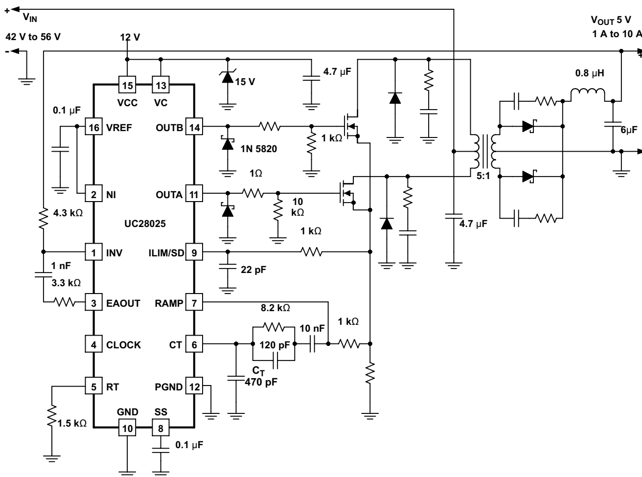
Figure 18. DC-DC Push-Pull Converter Using UC28025
