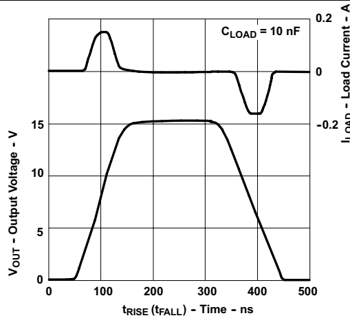
Figure 6. Rise and Fall Time vs Output Voltage and Load Current
