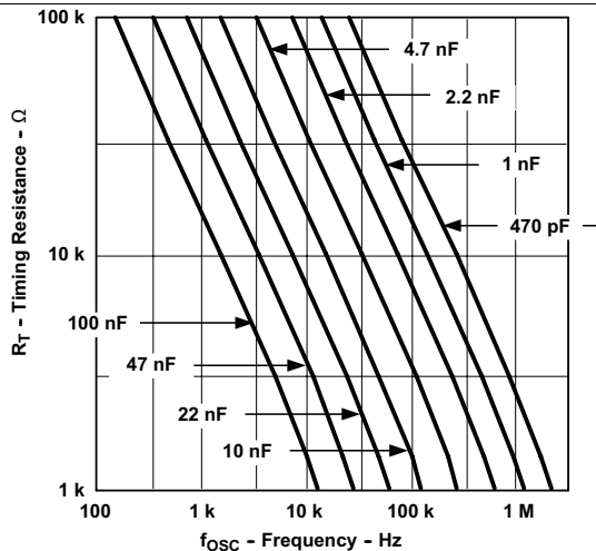
Figure 1. Timing Resistance vs Frequency
