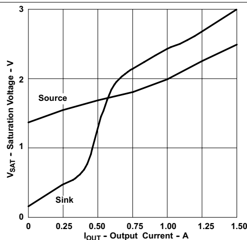
Figure 4. Saturation Voltage vs Output Current
