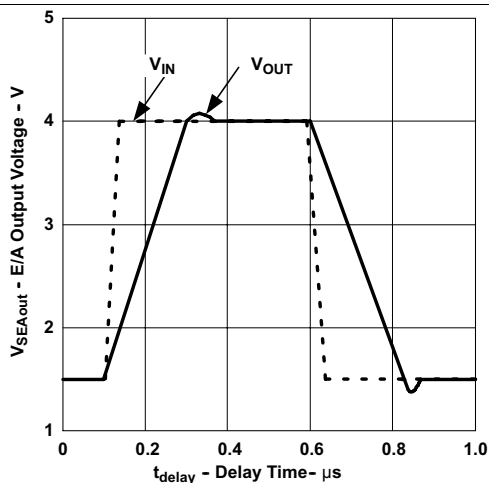
Figure 3. Unity Gain Slew Rate
