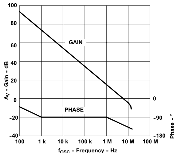
Figure 2. Open-Loop Frequency Response
