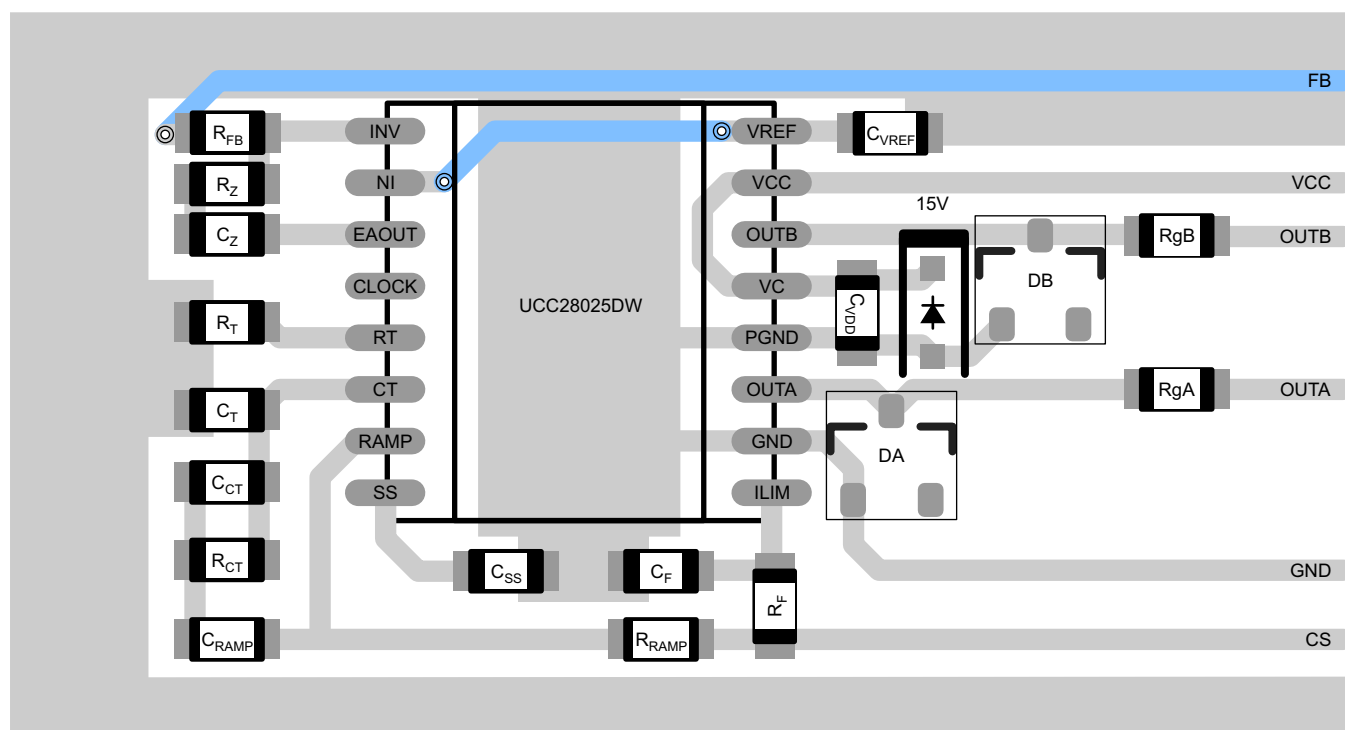
Figure 21. Layout Recommendation
