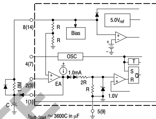
Figure 21. Soft-Start Circuit
