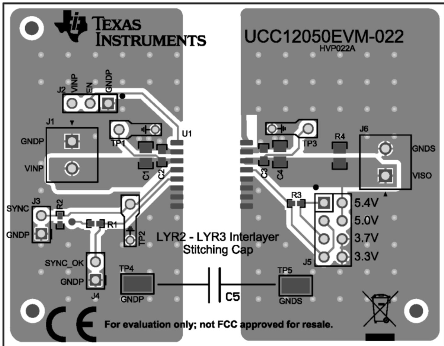
Figure 10-1. Layout Example
