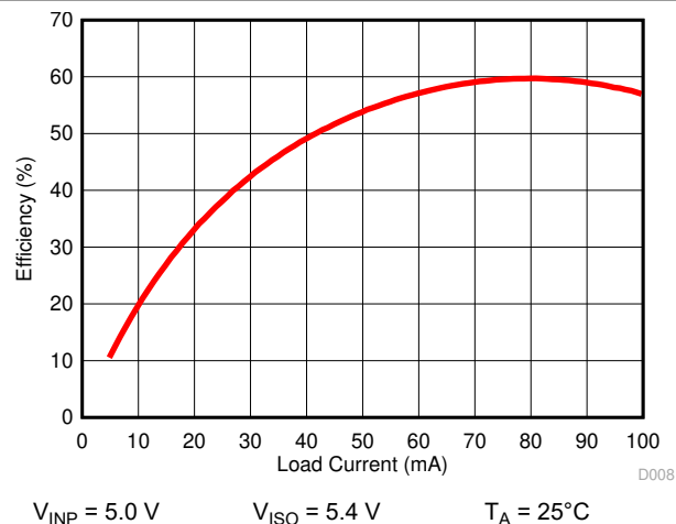
Figure 6-13. Power Supply Efficiency vs Load Current ( I_{ISO} )
