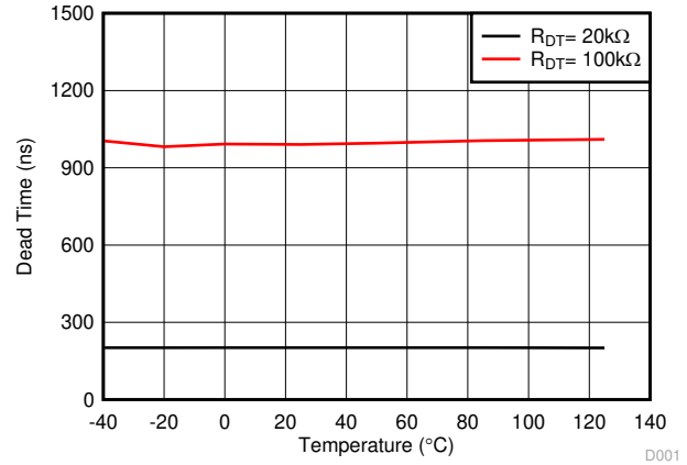
Figure 6-29. Dead Time vs. Temperature (with R_{DT} = 20\text{ k}\Omega and 100\text{ k}\Omega )
