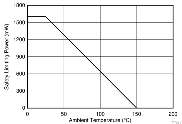
Figure 6-3. Thermal Derating Curve for Safety-Related Limiting Power
