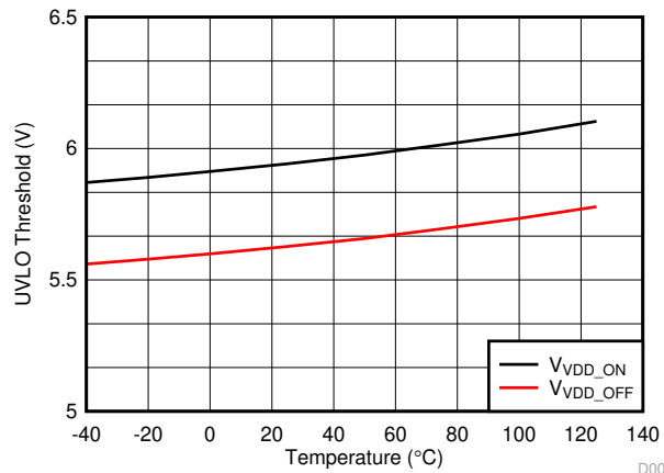
Figure 6-18. UCC21521ADW UVLO Threshold vs. Temperature
