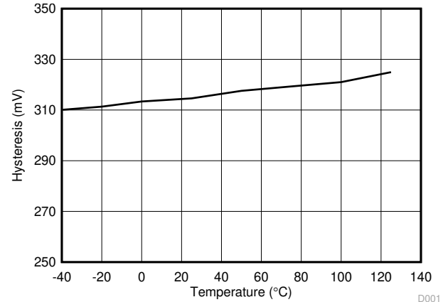
Figure 6-17. UCC21521ADW UVLO Hysteresis vs. Temperature
