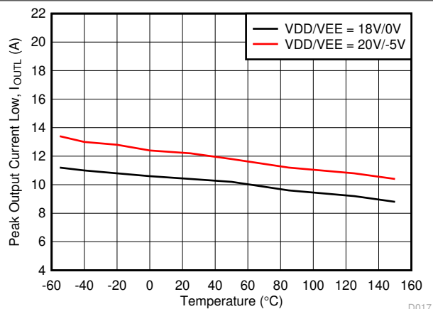
Figure 5-5. Output Low Driver Current vs. Temperature
