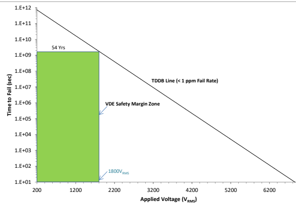
Figure 5-3. Reinforced Isolation Capacitor Life Time Projection
