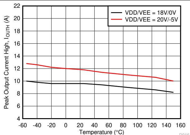
Figure 5-4. Output High Drive Current vs. Temperature
