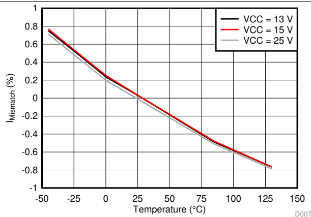
Figure 7. I_{\text{MISMATCH}} vs Temperature
