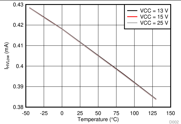
Figure 2. I HVLow vs Temperature
