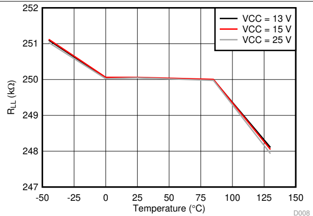
Figure 8. R_{\text{LL}} vs Temperature
