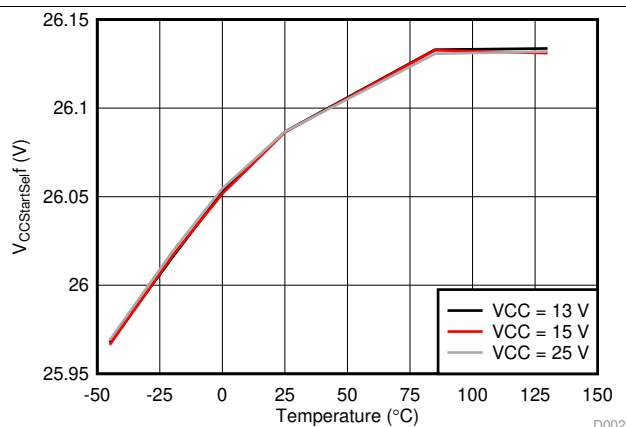
Figure 26. V_{CCStartSelf} vs Temperature
