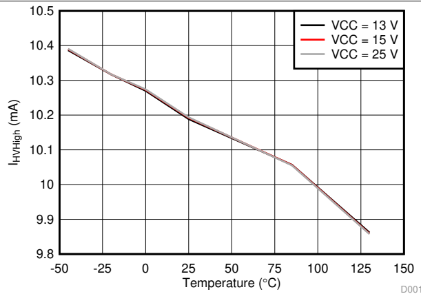
Figure 1. I HVHigh vs Temperature
