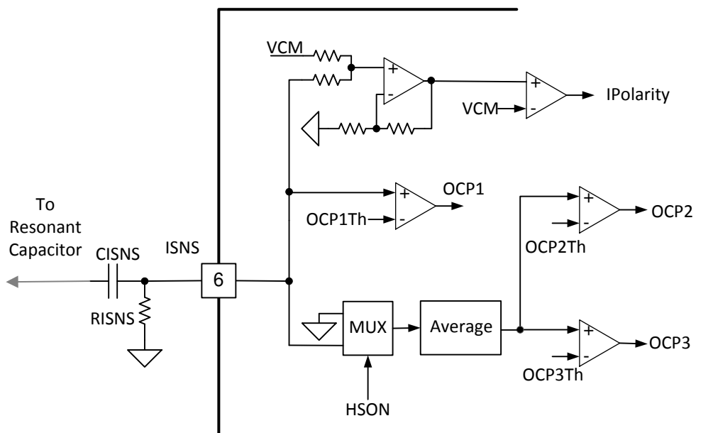
Figure 35. ISNS Block Diagram
