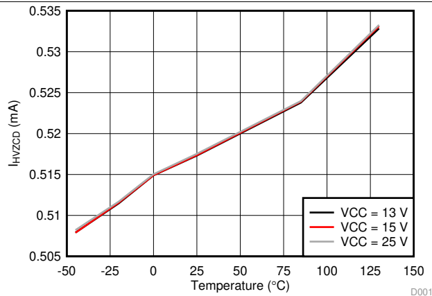
Figure 19. I_{HVZCD} vs Temperature
