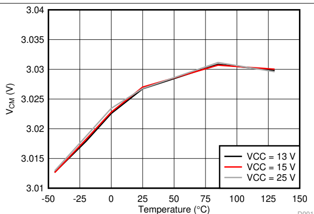
Figure 13. V_{CM} vs Temperature
