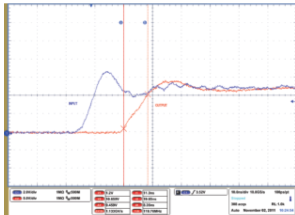
Figure 8-4. Typical Turnon Waveform
