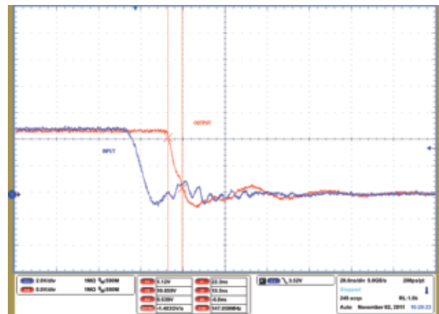
Figure 8-5. Typical Turnoff Waveform
