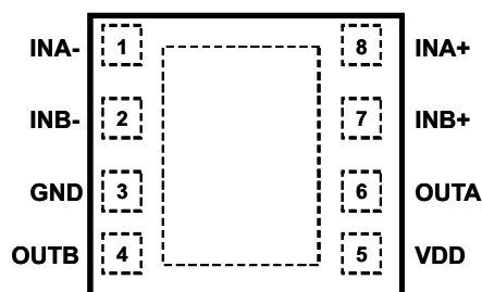
Figure 5-3. DSD Package UCC27526 8-Pin WSON Top View
