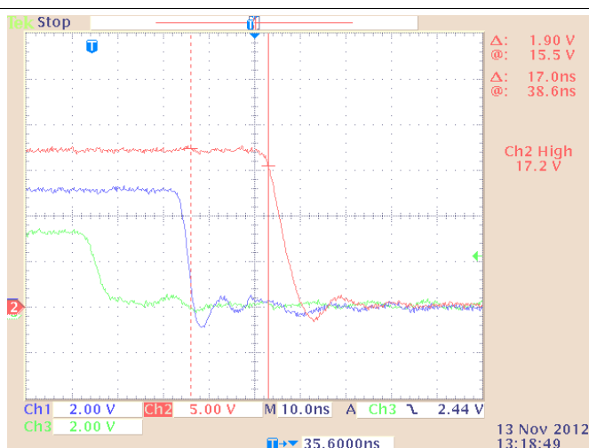
Figure 43. UCC27531DBV Input vs. Output PWM Propagation Delay (Low)
