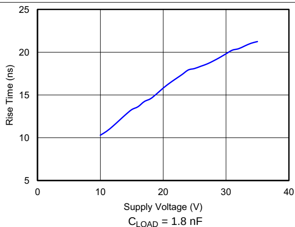
Figure 4. Rise Time vs. Supply Voltage
