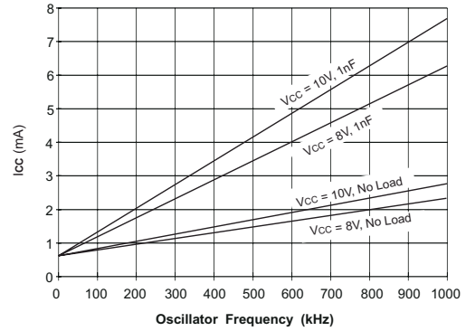
Figure 6-8. UCC2805-Q1 I CC vs Oscillator Frequency
