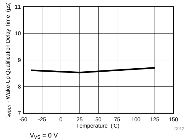
Figure 12. Wake-Up Qualification Delay Time vs. Temperature
