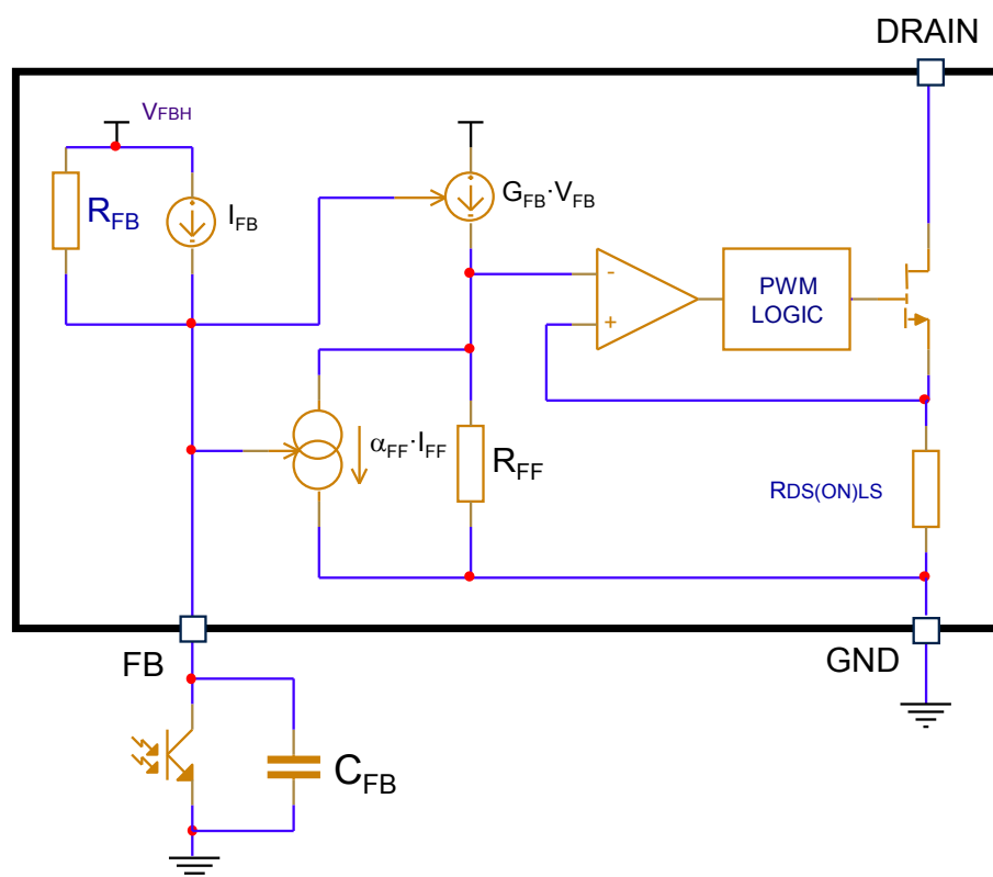
Figure 13. Constant output voltage control principle: internal schematic and pin configuration
