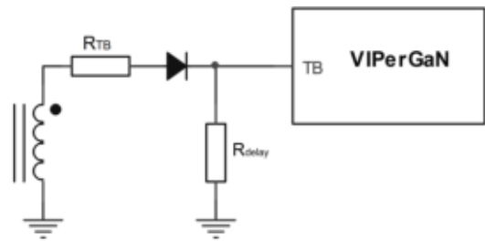
Figure 22. TB pin: external configuration: (only valley synch)
