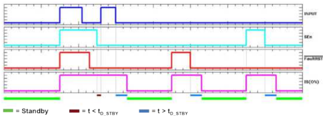
Figure 13. Standby state diagram
