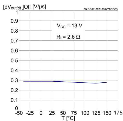
Figure 27. Turn-off voltage slope
