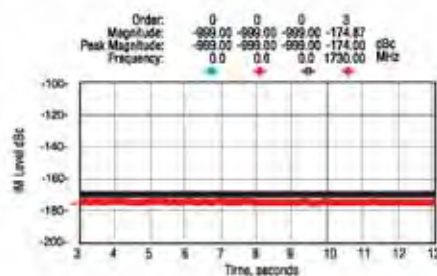
Dynamic PIM Test Results
