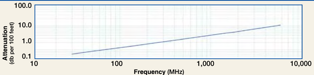
Attenuation vs. Frequency (typical)
