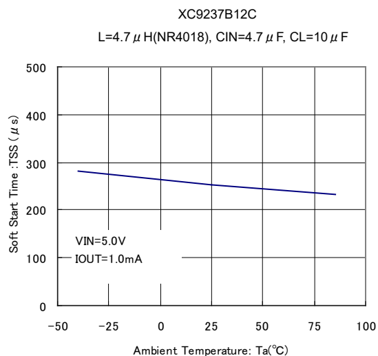
(13) XC9235B/36B/37B Soft-Start Time vs. Ambient Temperature
