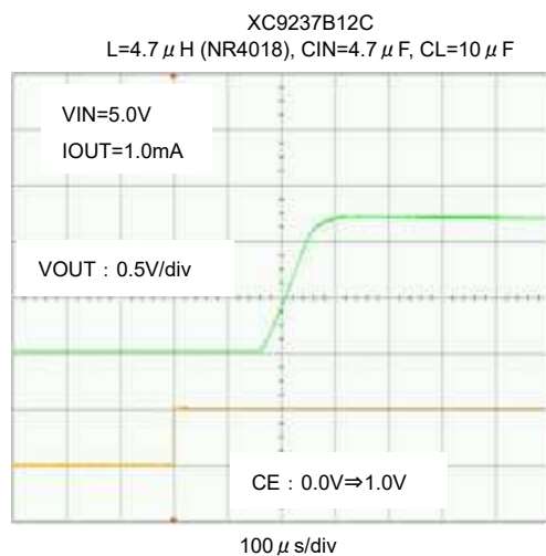
(12) XC9235B/36B/37B Rise Wave Form
