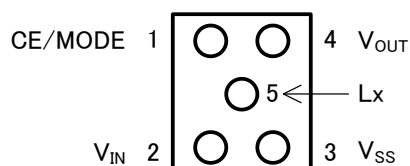
WLP-5-03 (BOTTOM VIEW)
