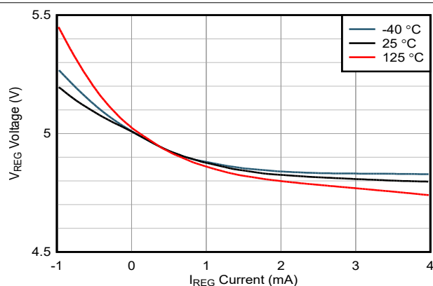
Figure 6-6. V_{\text{REG}} Voltage vs V_{\text{REG}} Current
